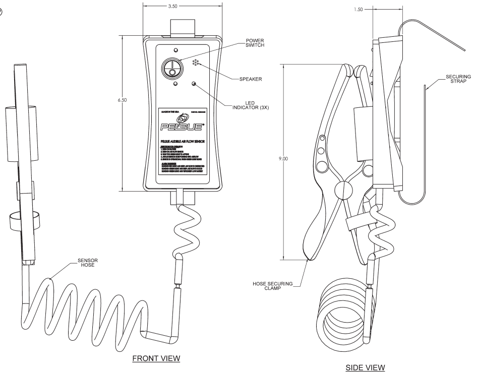
SIDE VIEW
