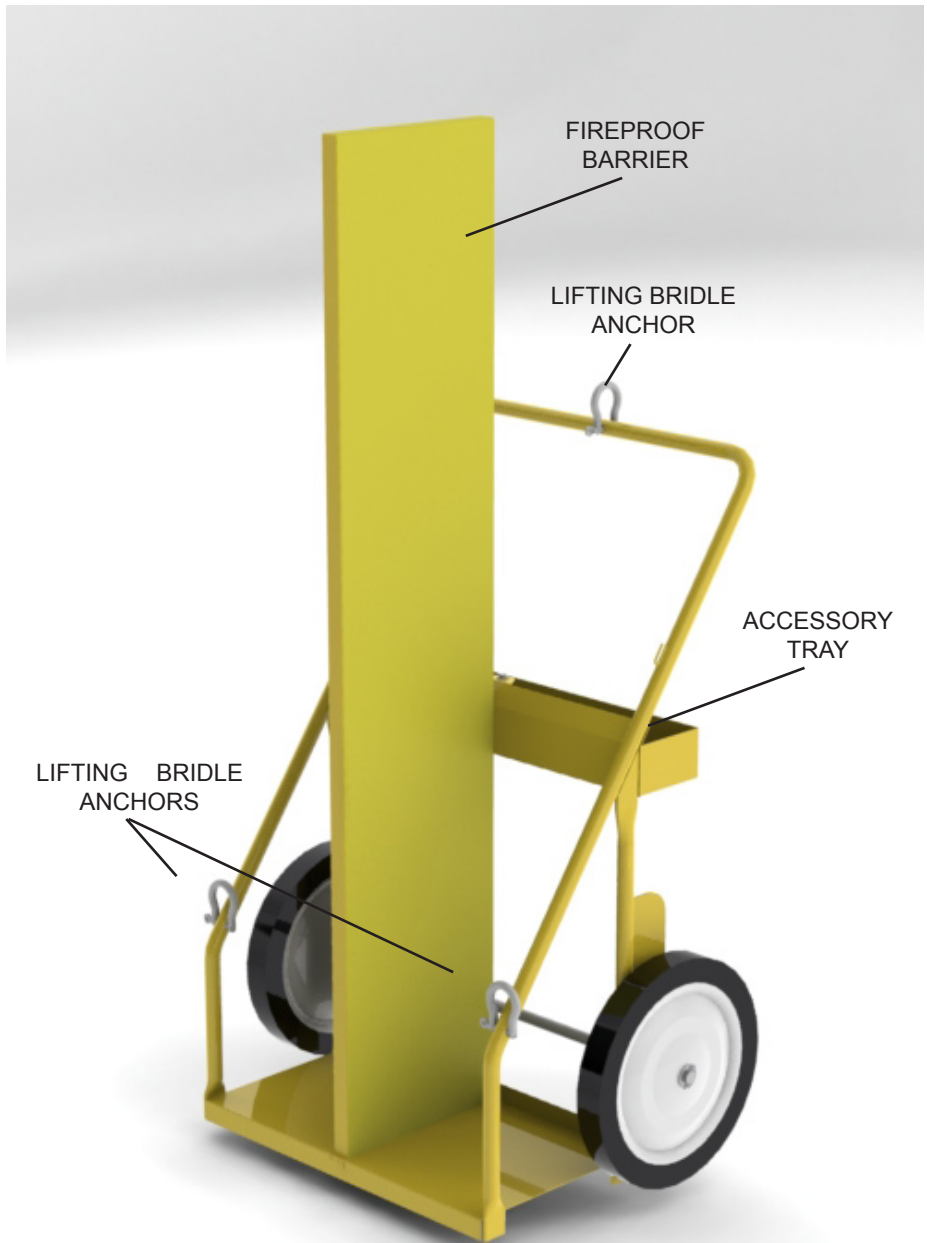
Welding Gas Cylinder Cart Isometric View
